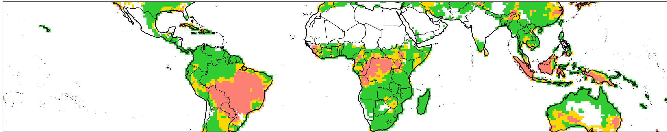
NCEP-CFSv2 forecast trigger probabilities for 2026 MAM
